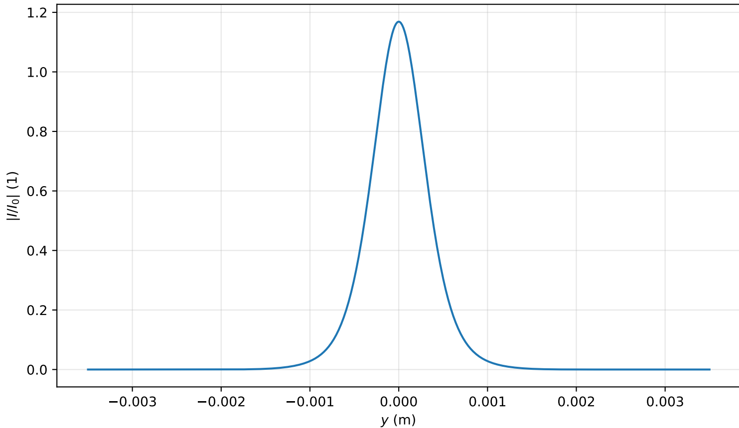
Intensity profile I(x=0, y, z=1.672)/I_0 , P_{in}=0.7P_{cr} , artificial time
